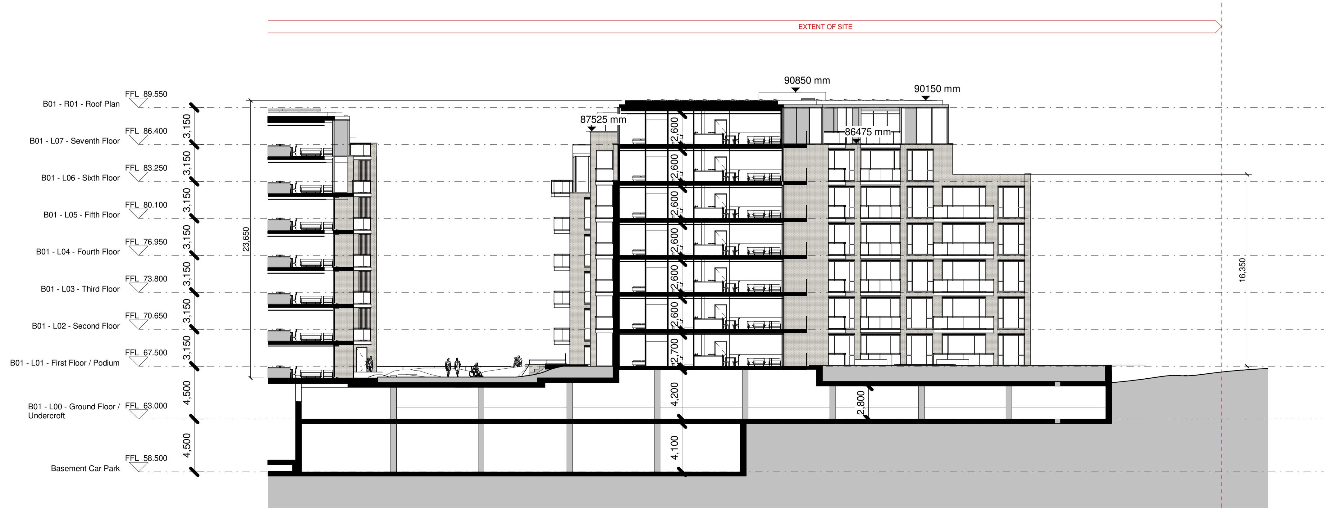
B Proposed Building 01 - Section B-B 1 : 200
