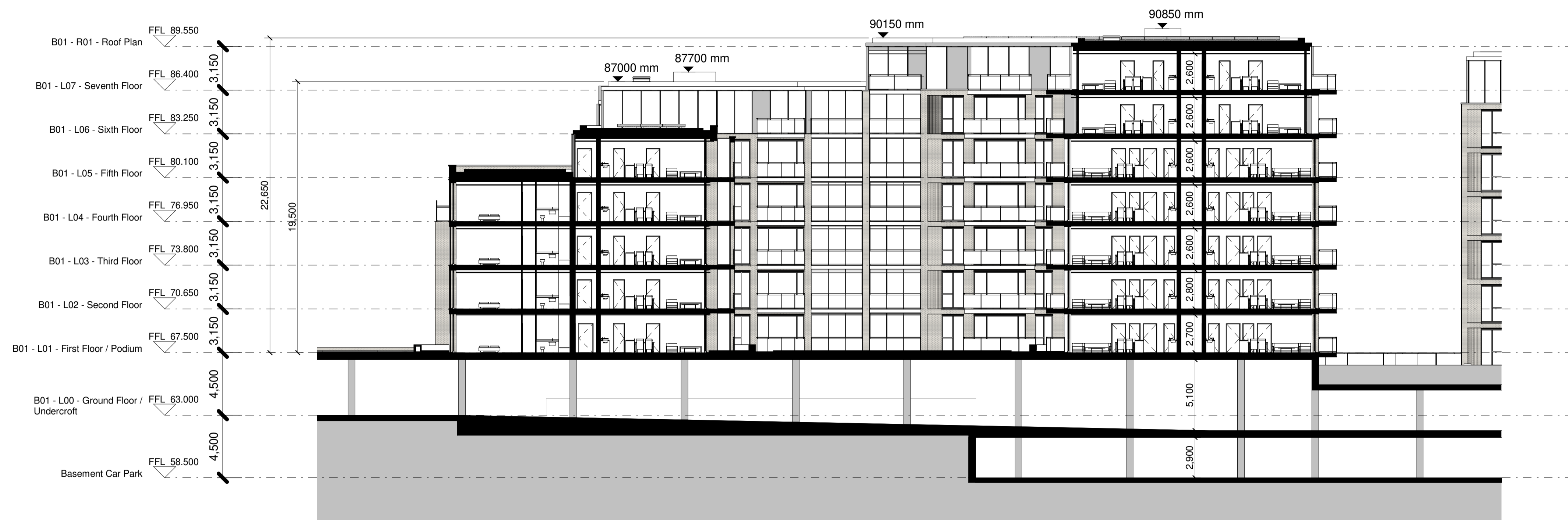
A Proposed Building 01 - Section A-A 1 : 200
