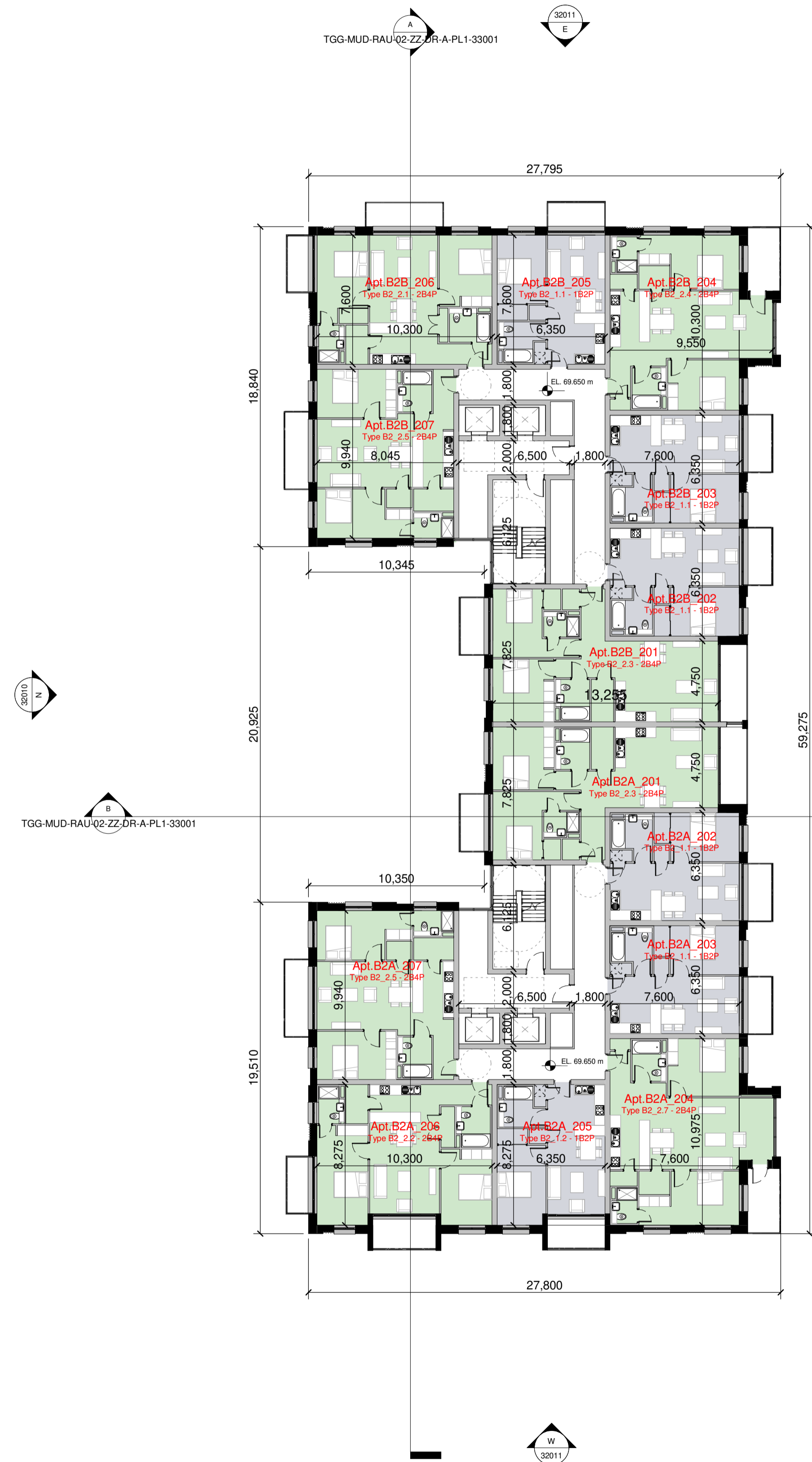
2 Proposed Building 02 - L02 - Second Floor Plan 1 : 200
