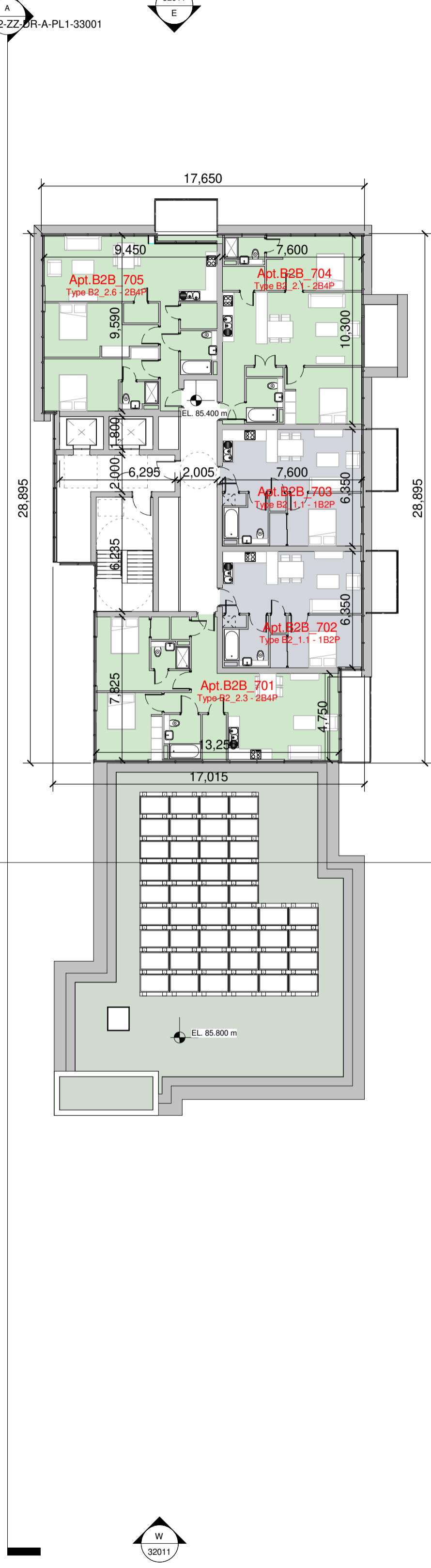
7 Proposed Building 02 - L07 - Seventh Floor Plan 1 : 200
