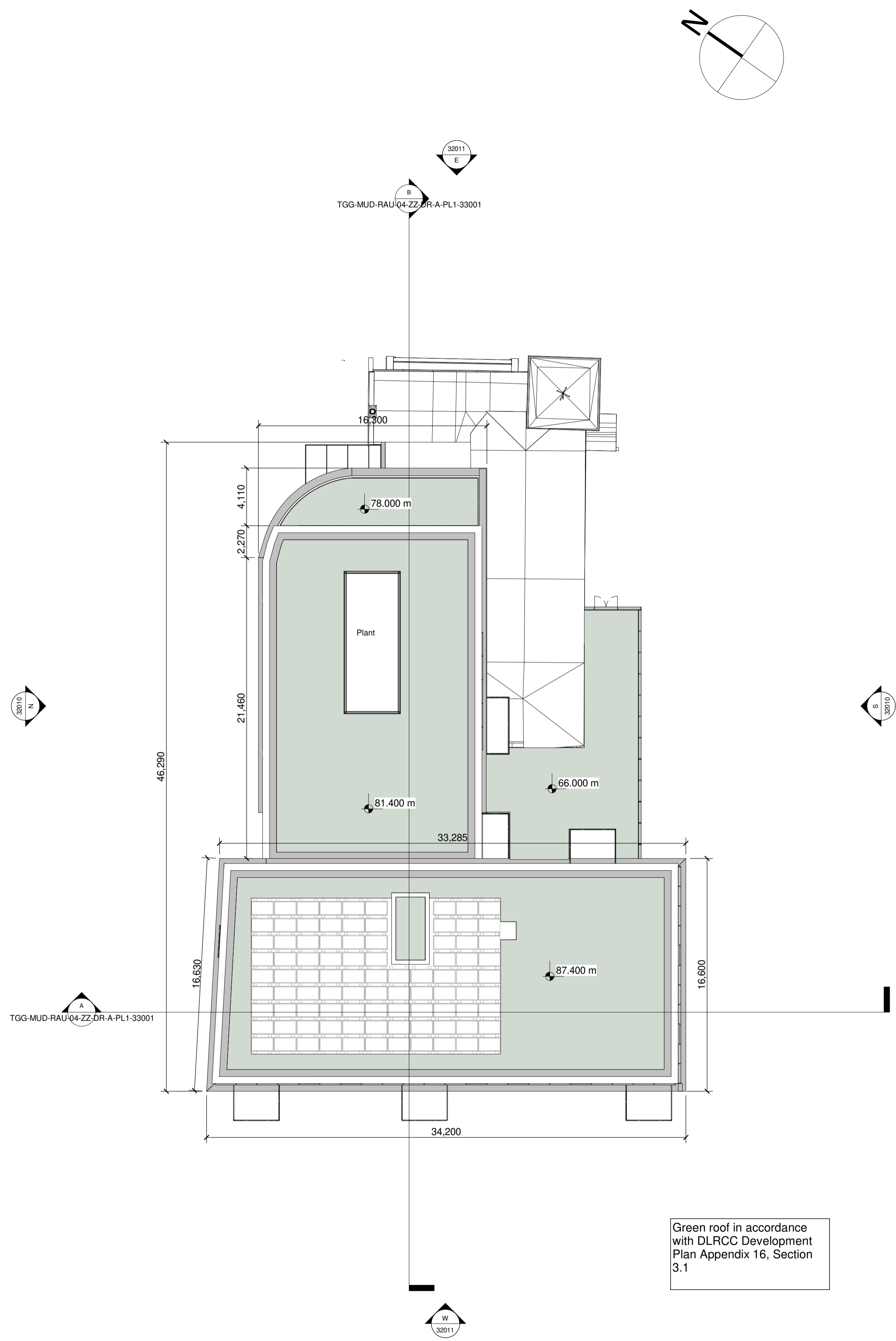
R Proposed Building 04 - R01 - Roof Plan 1 : 200
