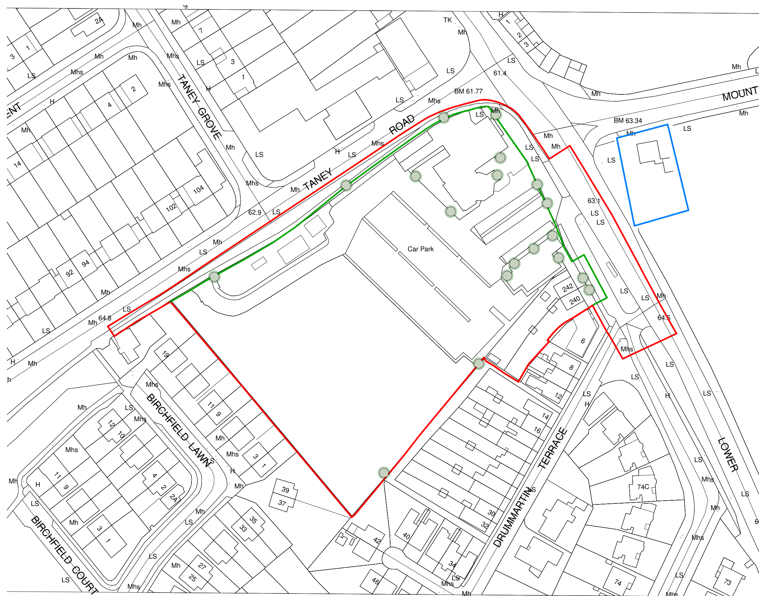
1 Site Location Plan 1 : 1000
