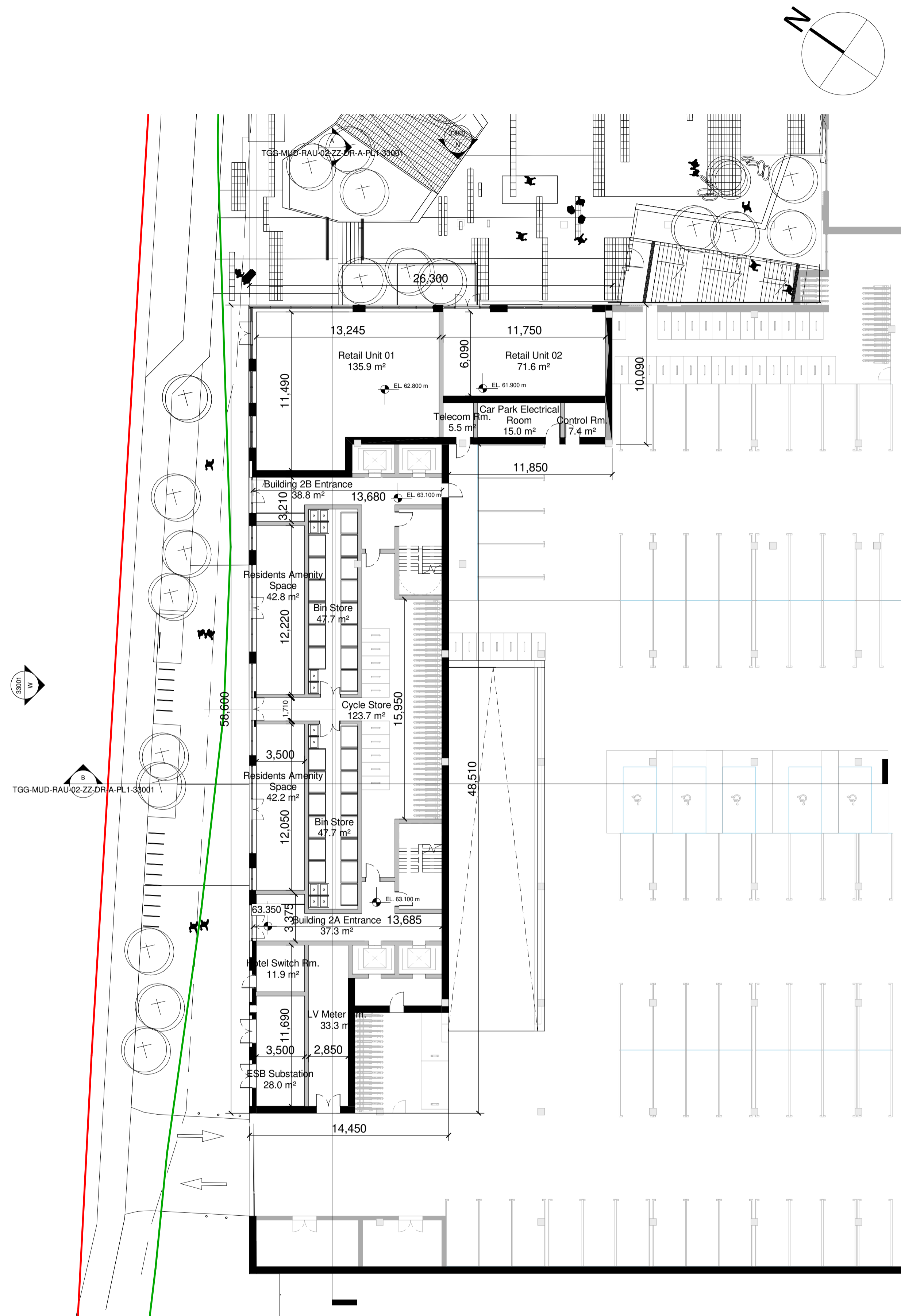
G Proposed Building 02 - L00 - Ground Floor / Undercroft Plan 1 : 200
