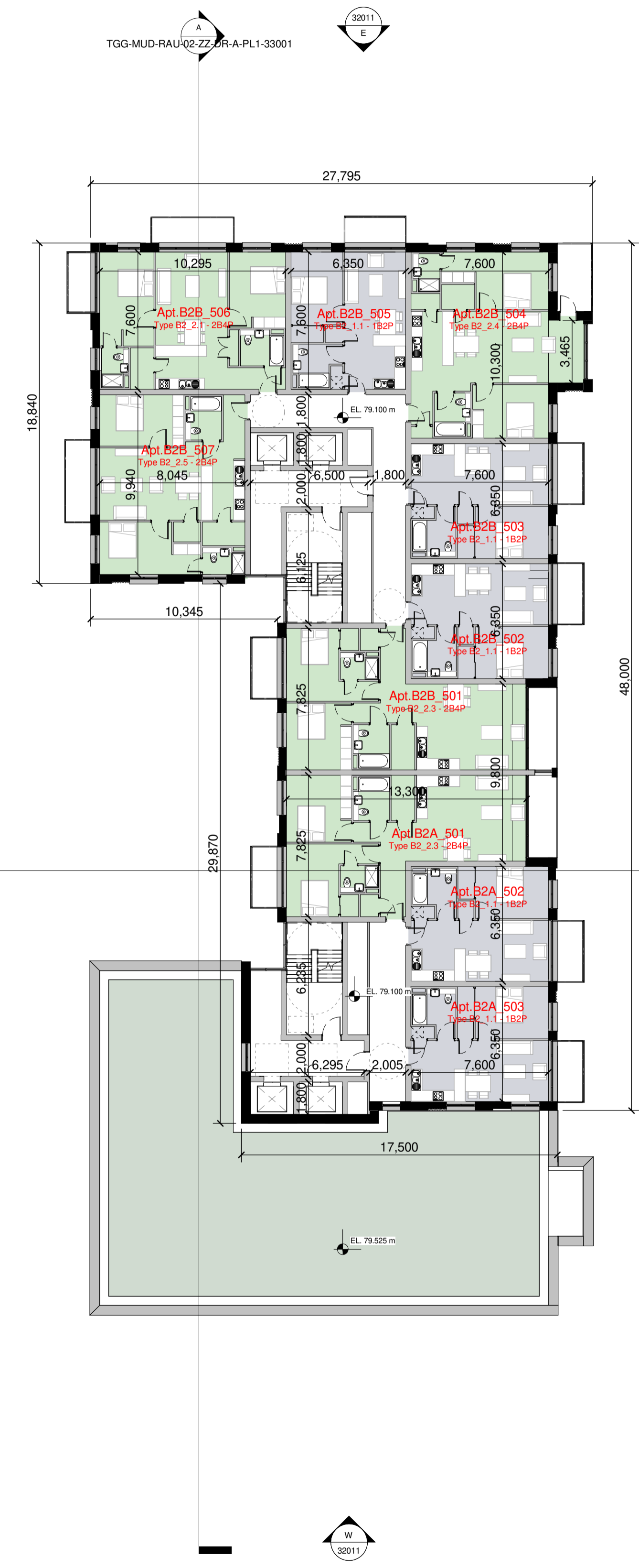
5 Proposed Building 02 - L05 - Fifth Floor Plan 1 : 200
