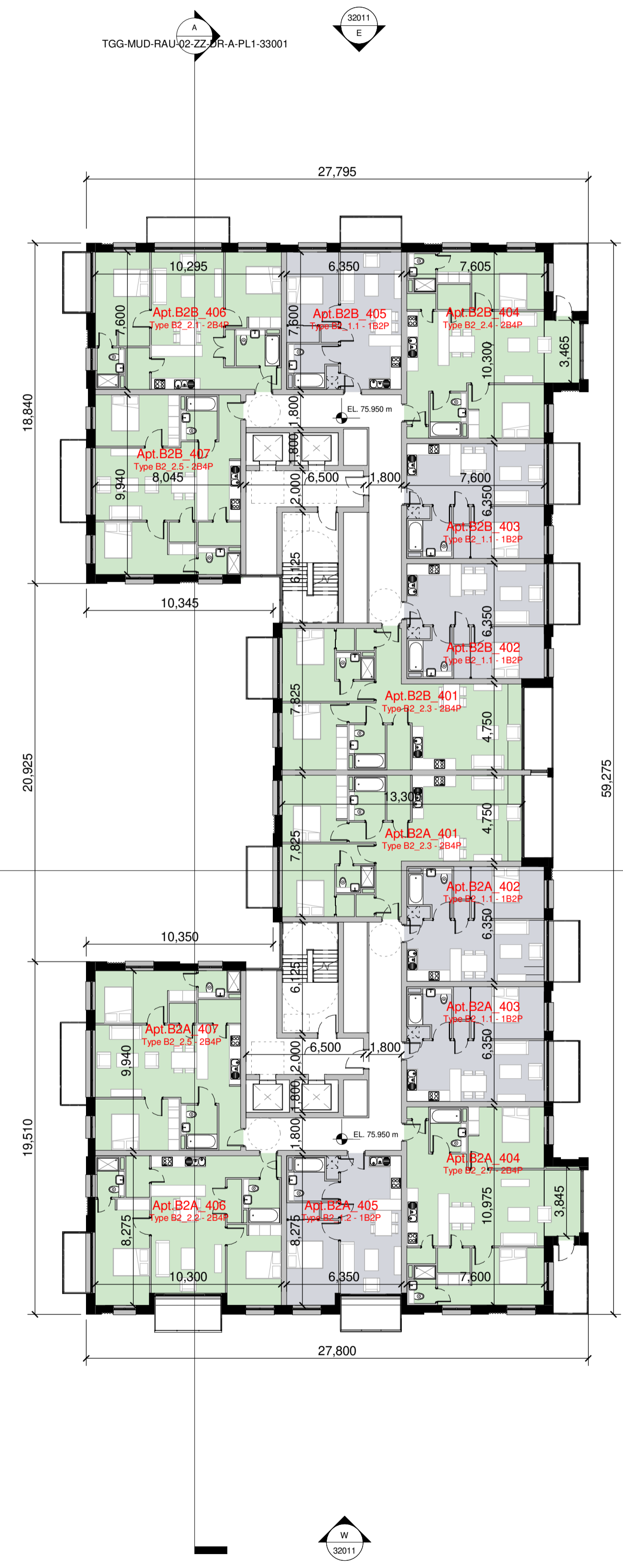
4 Proposed Building 02 - L04 - Fourth Floor Plan 1 : 200
